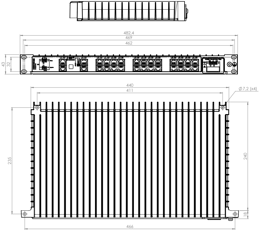
Figure 9. Dimensional drawing
