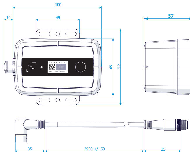
Figure 4.2: Neon Transmitter
