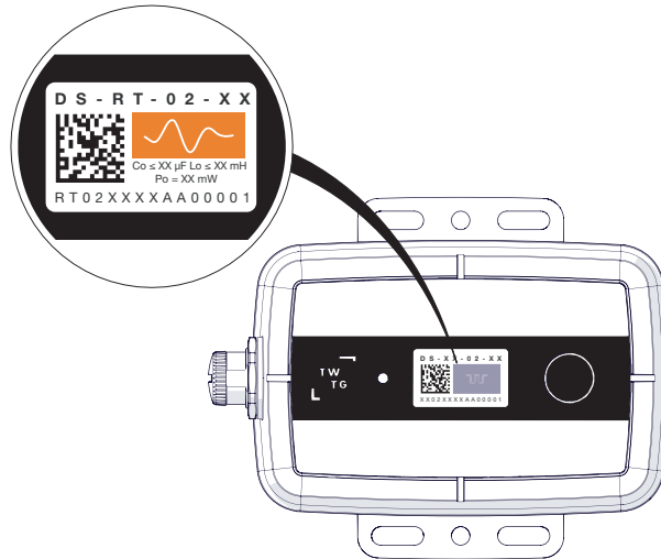
Figure 4.1: NFC and Data Matrix Code location
