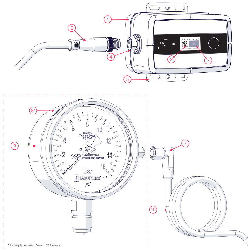
Figure 4.3: Component Names
