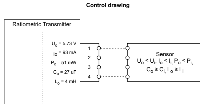
Figure 5.1: Intrinsic Safety Limiting Values
