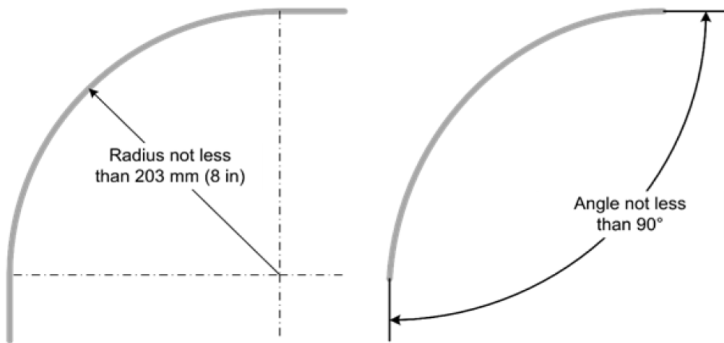
Figure 4: Grounding cable minimum bend radius and angle
