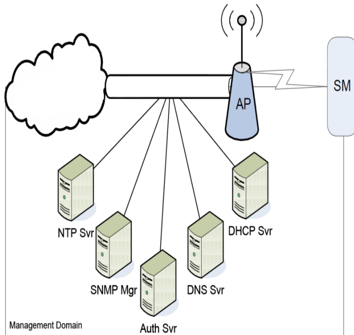
Figure 13: Cambium networks management domain
