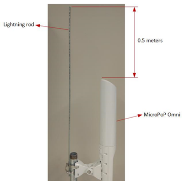
Figure 9: MicroPoP Omni with Lightning rod
