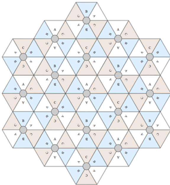
Figure 8: Example layout of 6 Access Point sectors (ABC), 60-degree sectors
