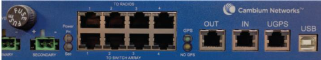
Figure 22: Injector Module
