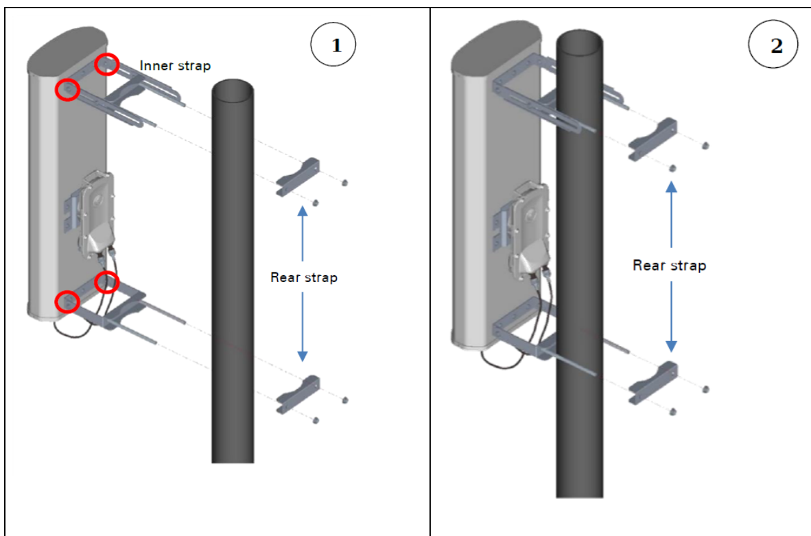
Figure 37: Attaching radio mounting PMP 450i AP 900 MHz antenna to the pole
