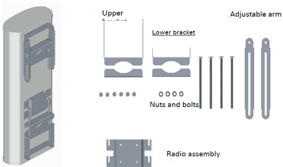
Figure 36: PMP 450i AP 900 MHz antenna inventory
