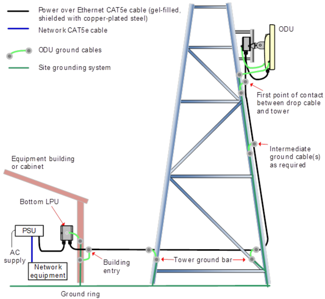
Figure 1: Mast or tower installation
