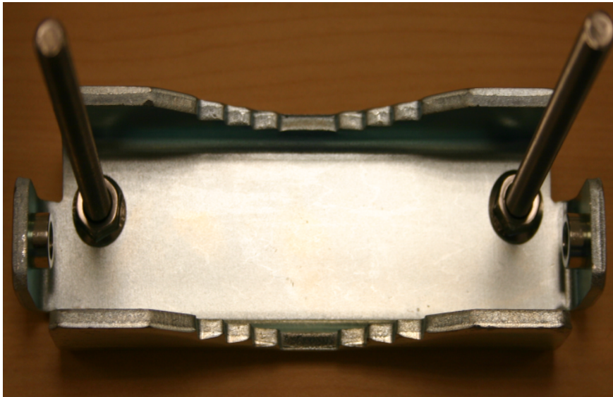
Figure 23: AP antenna upper bracket assembly
