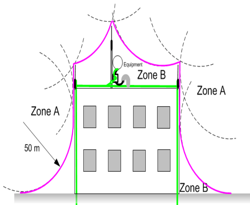
Figure 6: Rolling sphere method to determine the lightning protection zones
