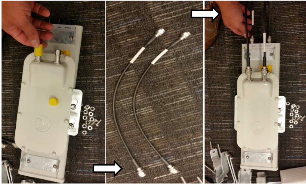
Figure 14: Connect the port A and B to the PMP 450i AP
