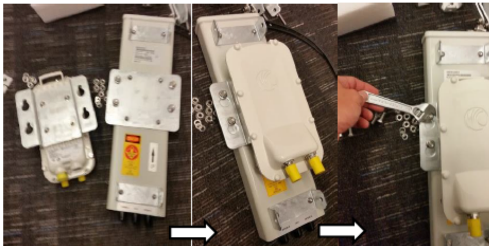
Figure 13: Attaching the plate
