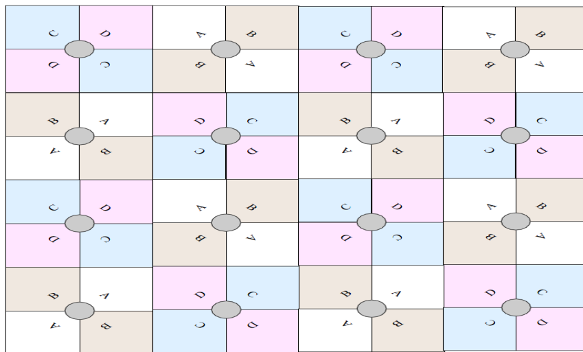
Figure 7: Example layout of 16 Access Point sectors (ABCD), 90-degree sectors
