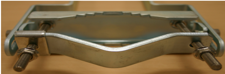
Figure 17: Rear strap connected to upper AP antenna bracket
