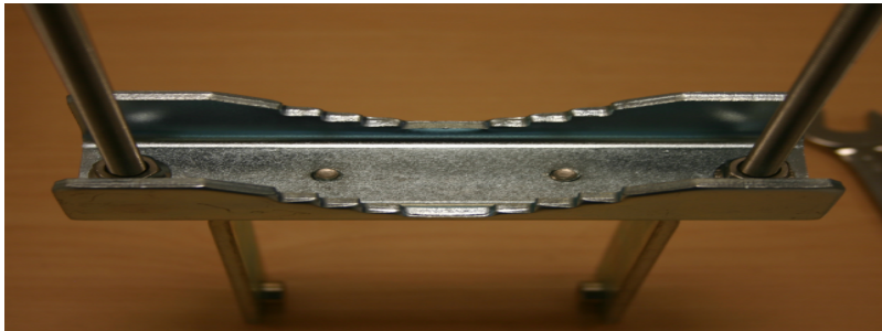
Figure 19: AP Antenna Lower Bracket Assembly
