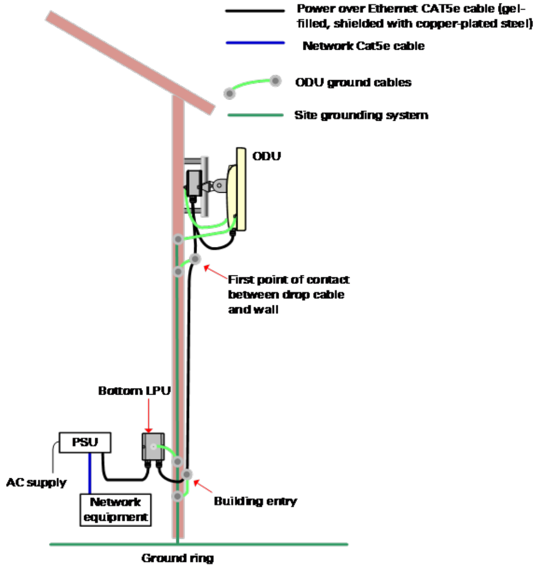
Figure 2: Wall installation
