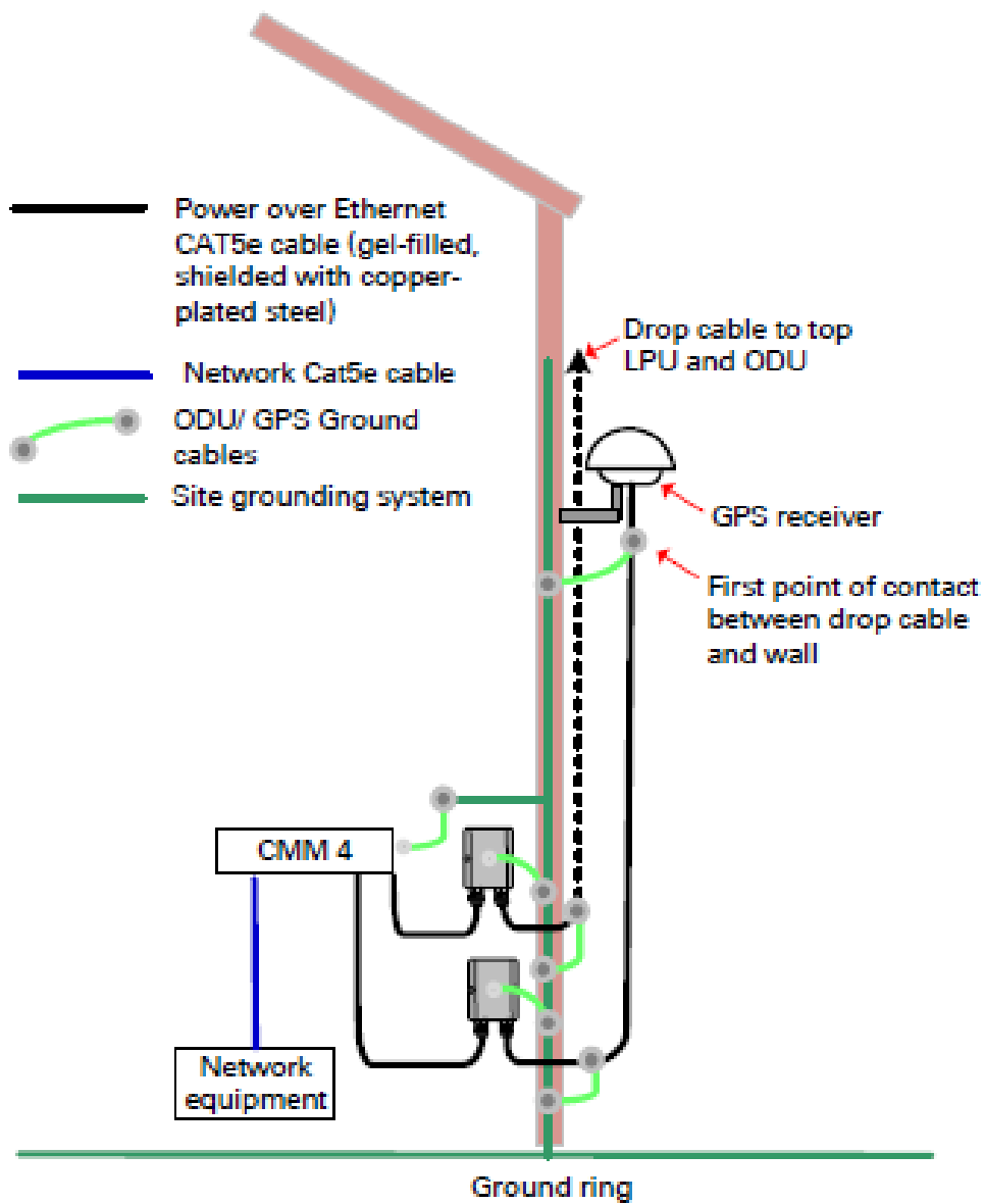
Figure 4: GPS receiver wall installation
