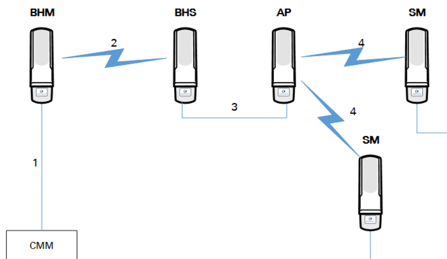
Figure 22: Additional link to extend network sync, Design 5
