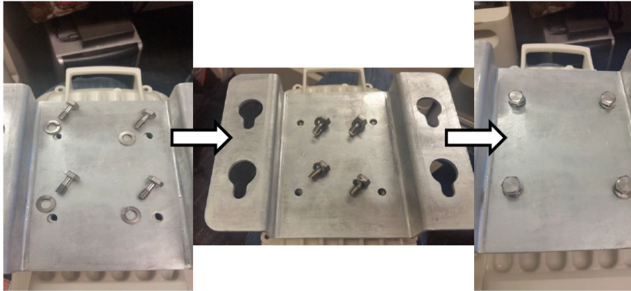
Figure 12: Attaching antenna plate to the AP
