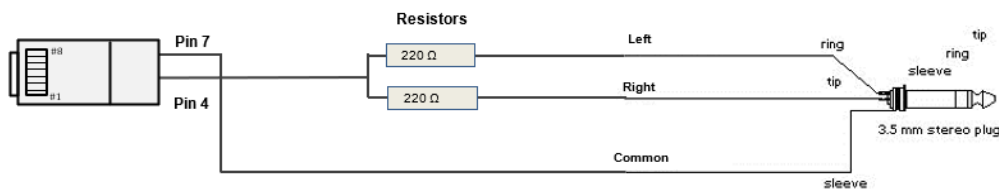
Figure 5: Alignment tone cable pin configuration
