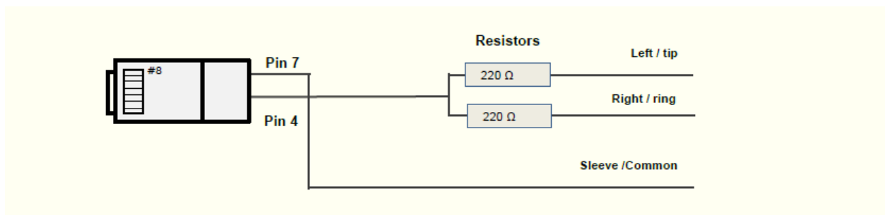
Figure 13: Alignment Tone Cable
