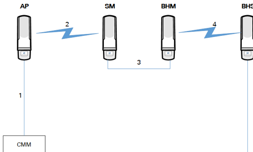
Figure 21: Additional link to extend network sync, Design 4
