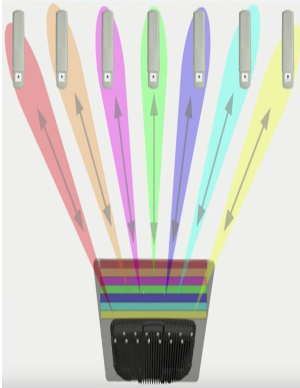
Figure 12: PMP 450m Series AP antenna beam
