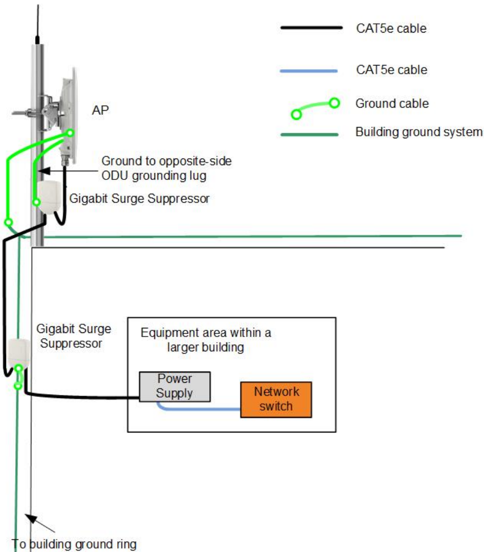
Figure 7: Grounding and lightning protection on building
