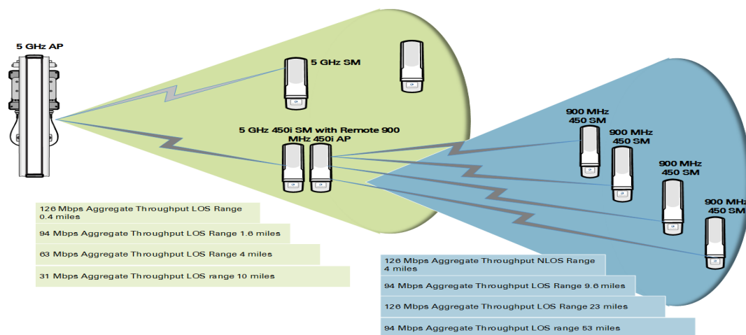
Figure 17: Example for 900-MHz remote AP behind 5 GHz SM
