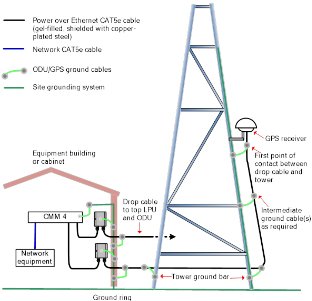
Figure 5: GPS receiver tower or mast installation
