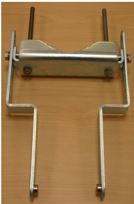
Figure 24: AP antenna upper bracket attached to upper adjustment arms
