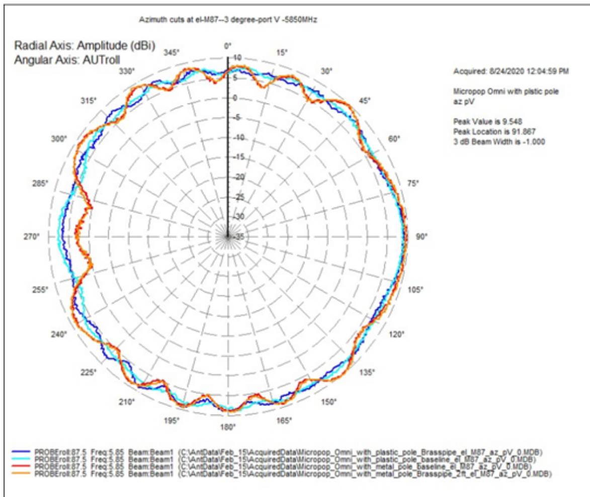
Figure 8: MicroPoP Omni antenna implementation pattern (Vertical)
