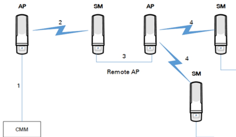
Figure 20: Additional link to extend network sync, Design 3
