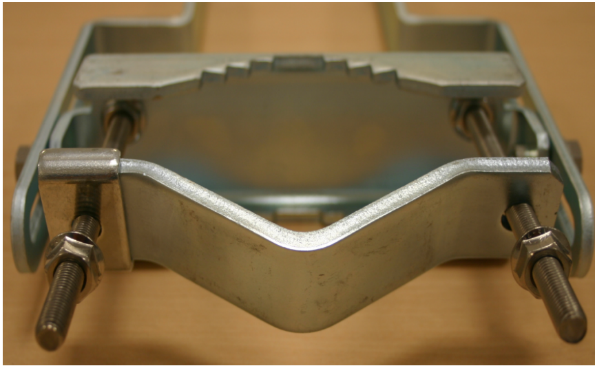
Figure 25: Rear strap connected to upper AP antenna bracket
