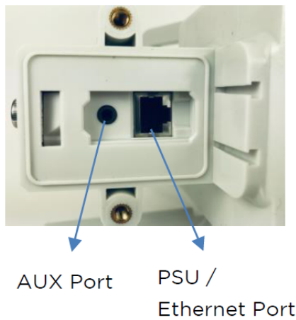
Figure 8: 3 GHz 450b Series interfaces (High Gain)
