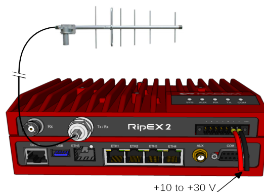
Fig. 4.10: 10–30 VDC Supplying
