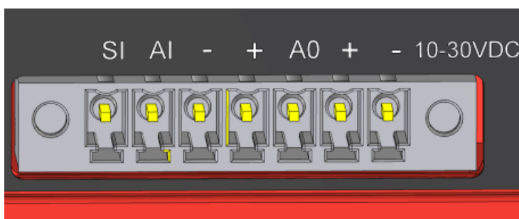
Fig. 2.7: Supply connector
