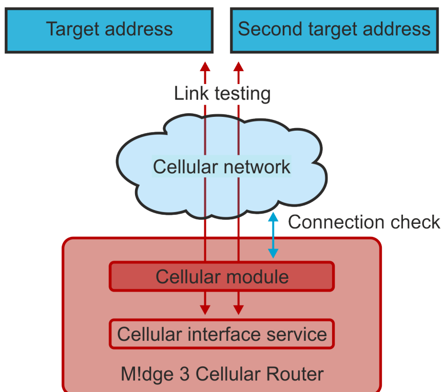
Fig. 7.4: Link testing scheme
