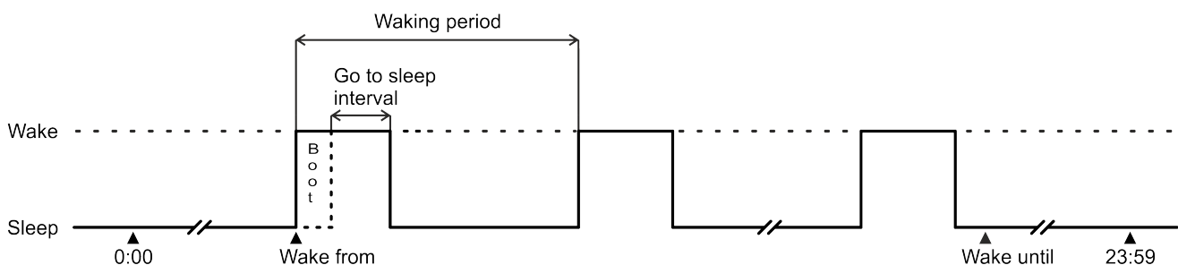
Fig. 7.26: Sleep mode scheme
