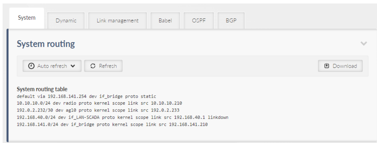
Fig. 8.2: DIAGNOSTICS > Information > Routing
