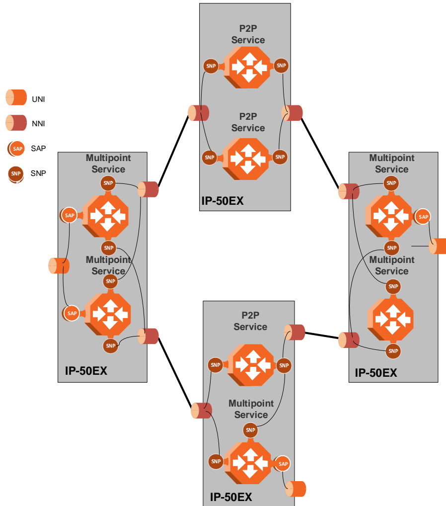
Figure 28: IP-50EX Services Model
