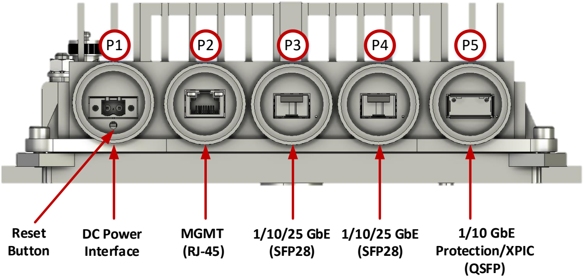
Figure 8: IP-50EX Interfaces
