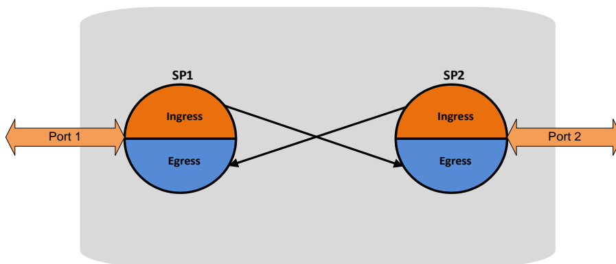
Figure 38: Service Path Relationship on Point-to-Point Service Path
