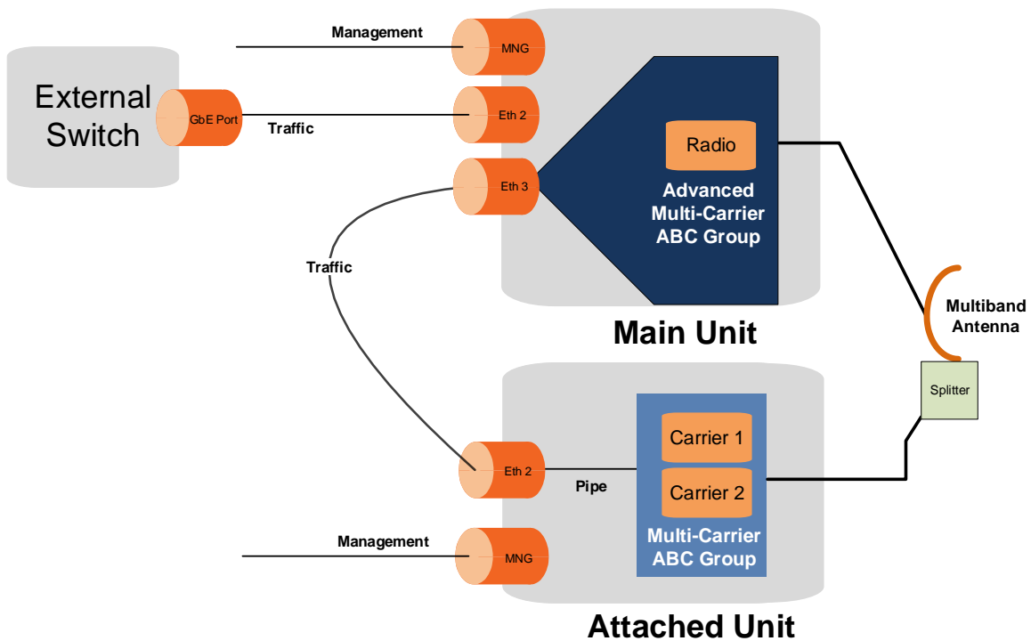
Figure 17: Layer 1 Link Aggregation (Multiband with Multiband Antenna)
