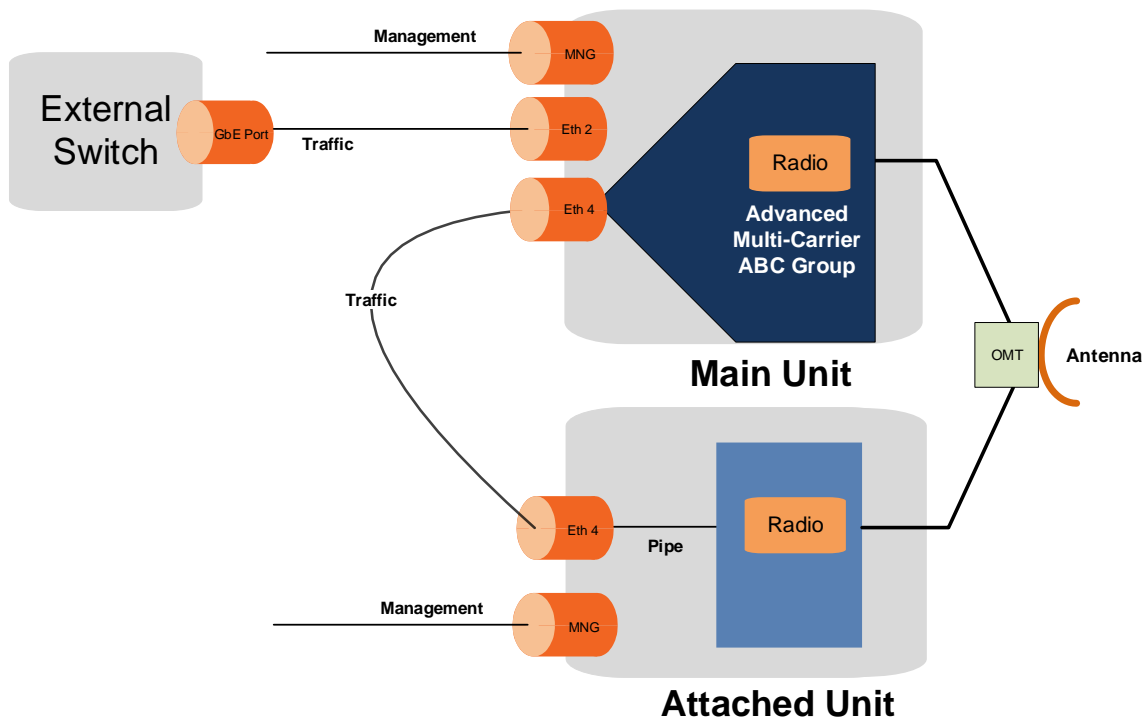
Figure 18: Layer 1 Link Aggregation (XPIC with Two IP-50EXA Devices)
