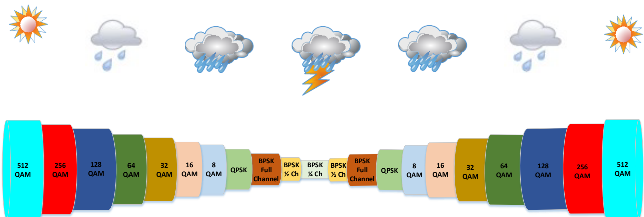
Figure 16: Adaptive Coding and Modulation with Eleven Working Points
