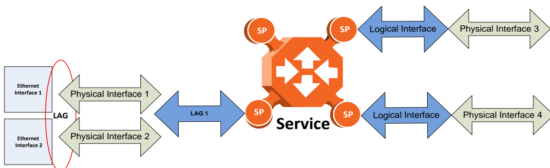
Figure 42: Relationship of Logical Interfaces to the Switching Fabric
