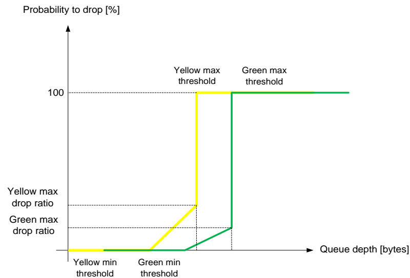
Figure 47: WRED Profile Curve
