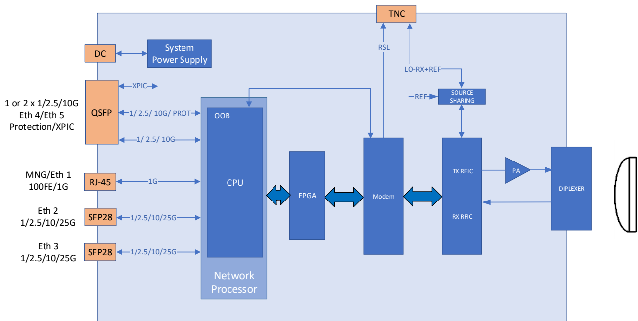
Figure 13: IP-50EXA Block Diagram
