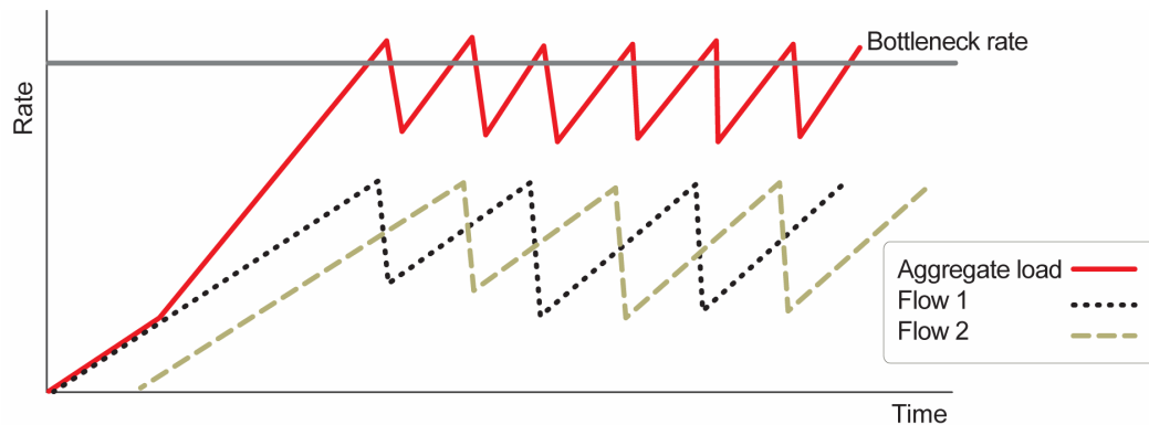
Figure 46: Random Packet Loss with Increased Capacity Utilization Using WRED
