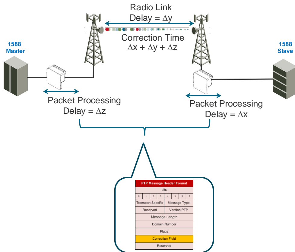
Figure 57: Transparent Clock Delay Compensation
