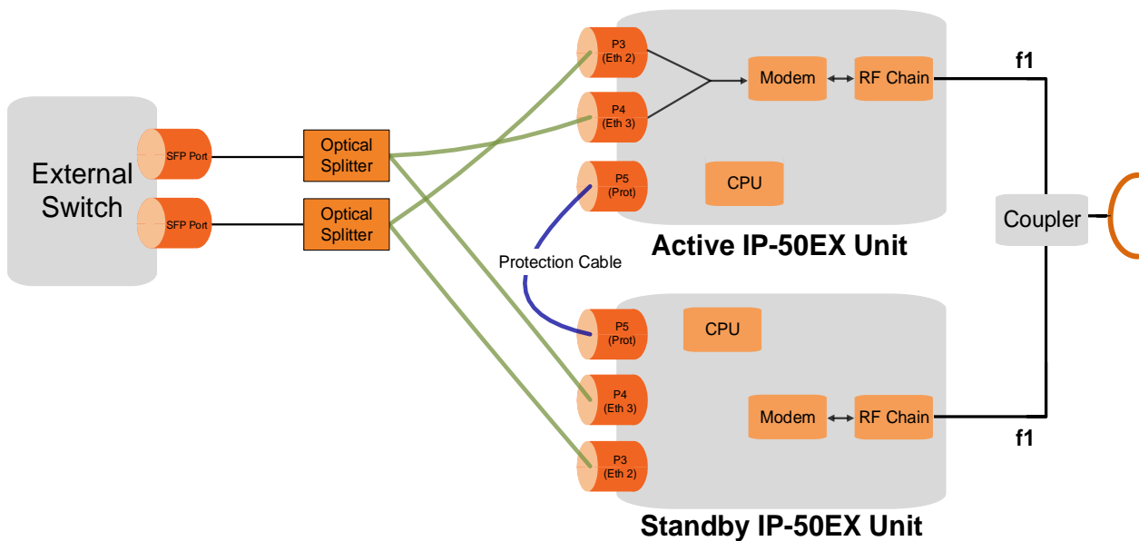
Figure 26: 1+1 HSB Unit Protection – Split Protection Mode
