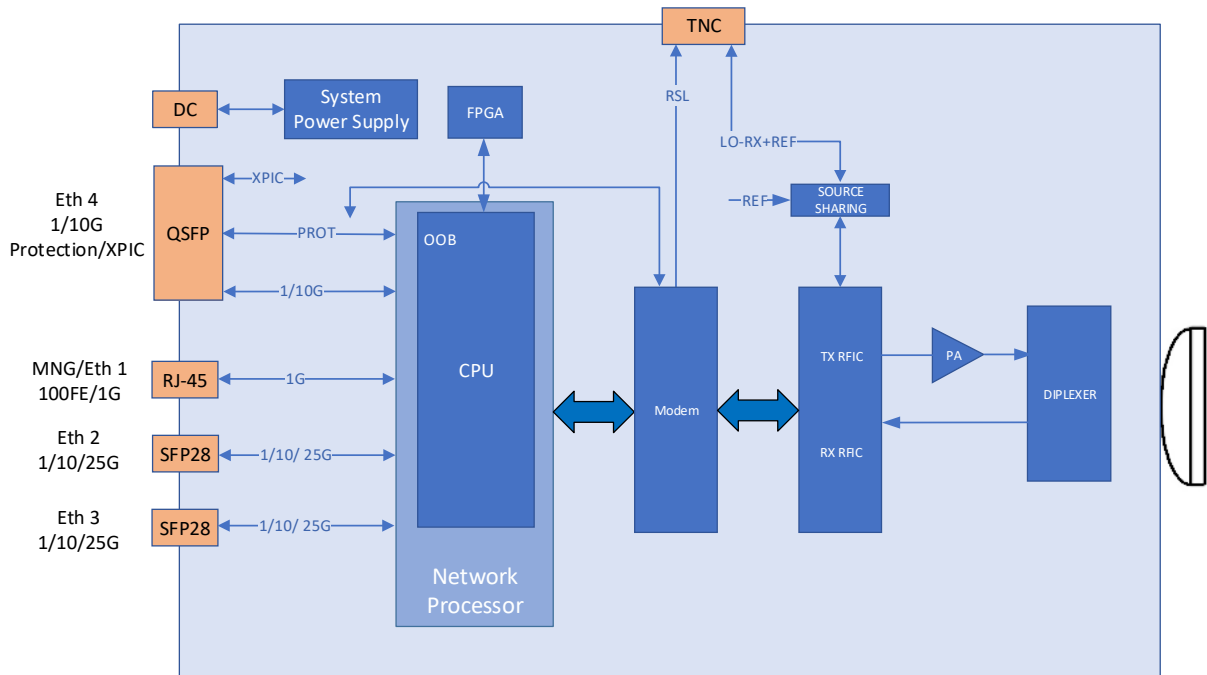
Figure 11: IP-50EX Block Diagram
