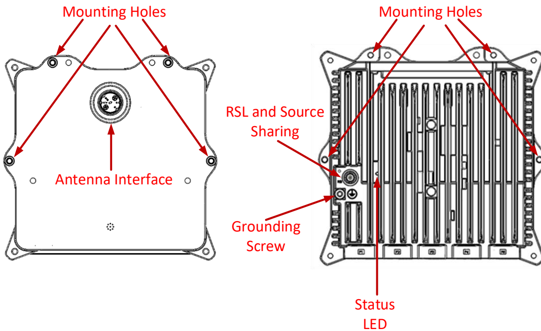
Figure 6: IP-50EX Direct Mount HW Ready – Rear View (Left) and Front View (Right)
