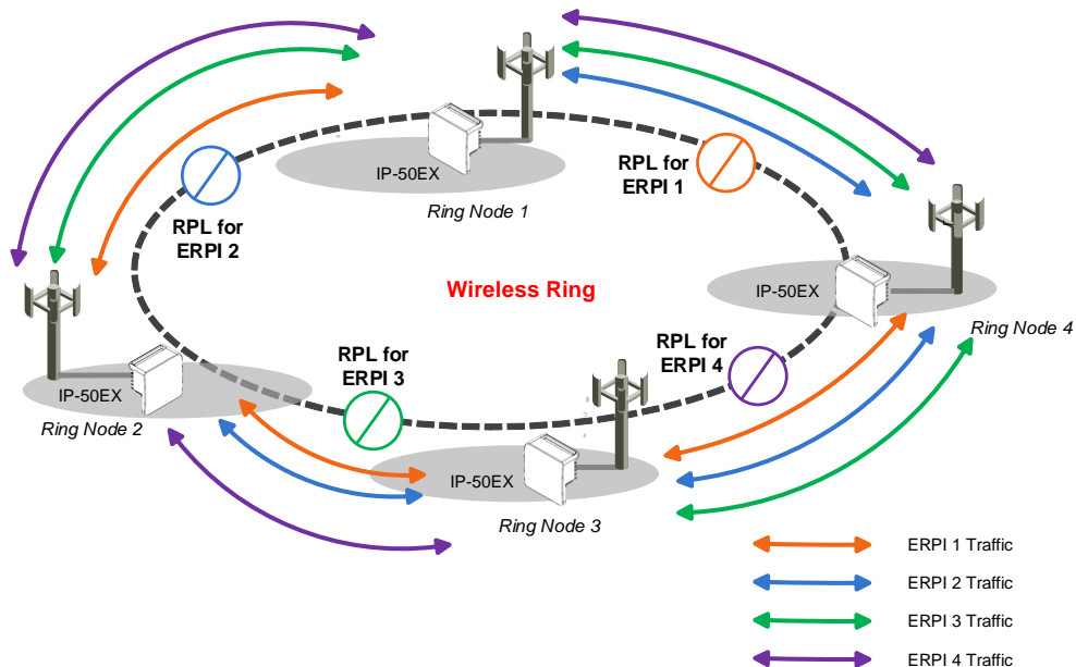
Figure 51: Load Balancing Example in G.8032 Ring
