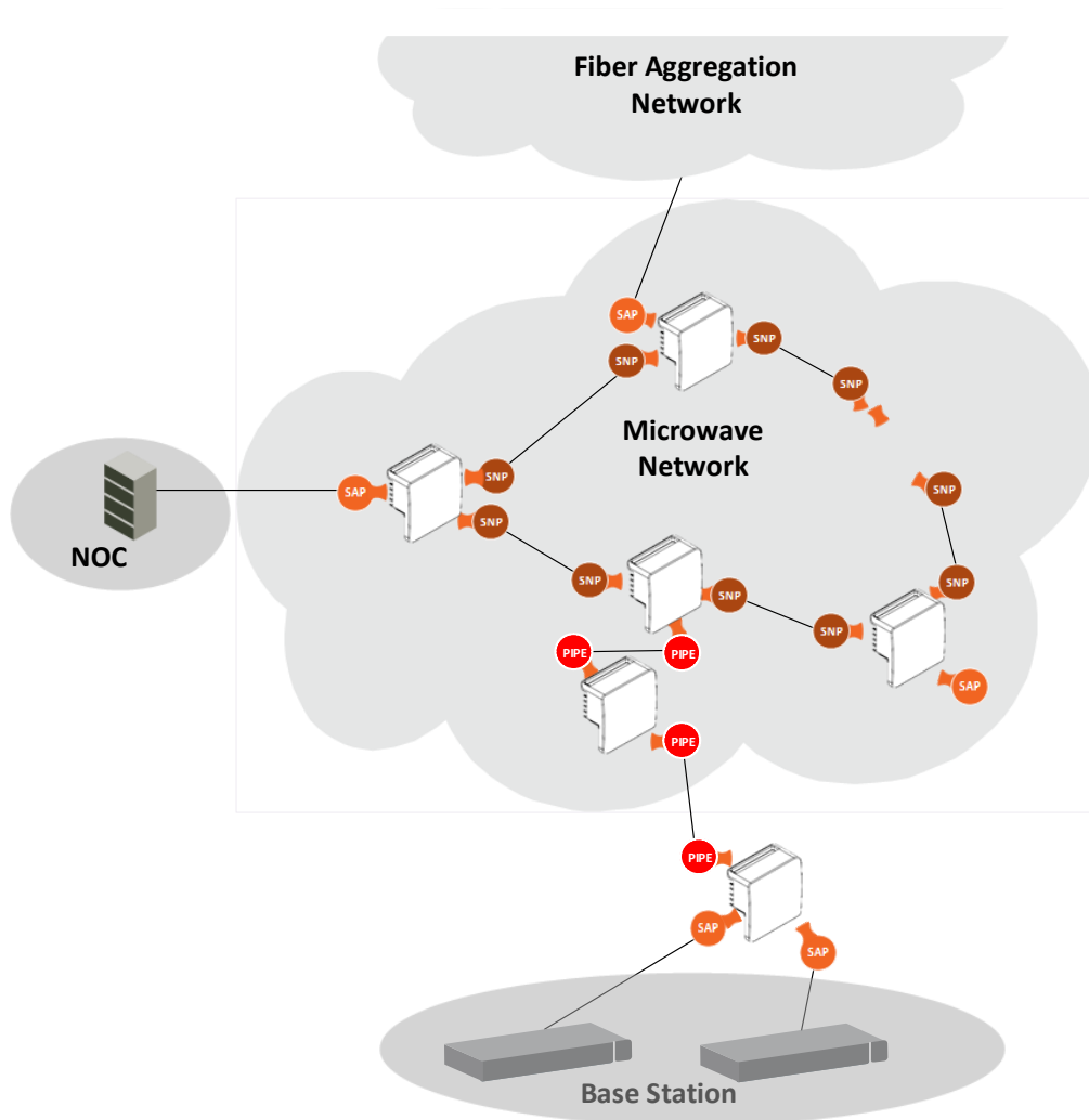
Figure 37: SAP, SNP and Pipe Service Points in a Microwave Network
