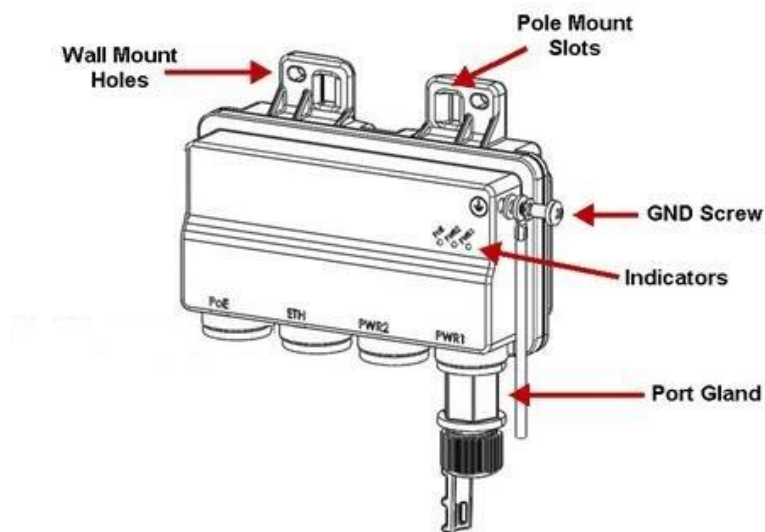
Figure 14: PoE Injector
