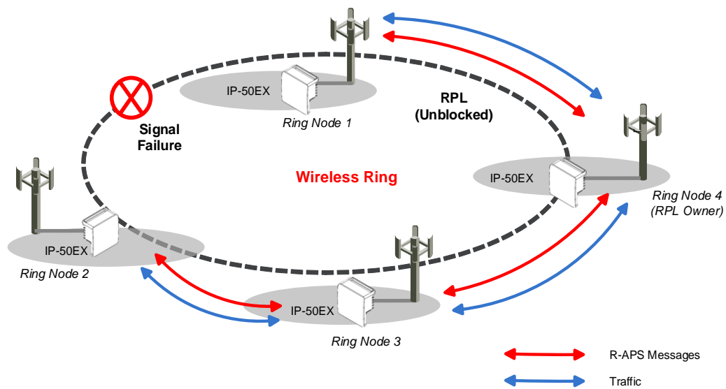
Figure 50: G.8032 Ring in Protecting State
