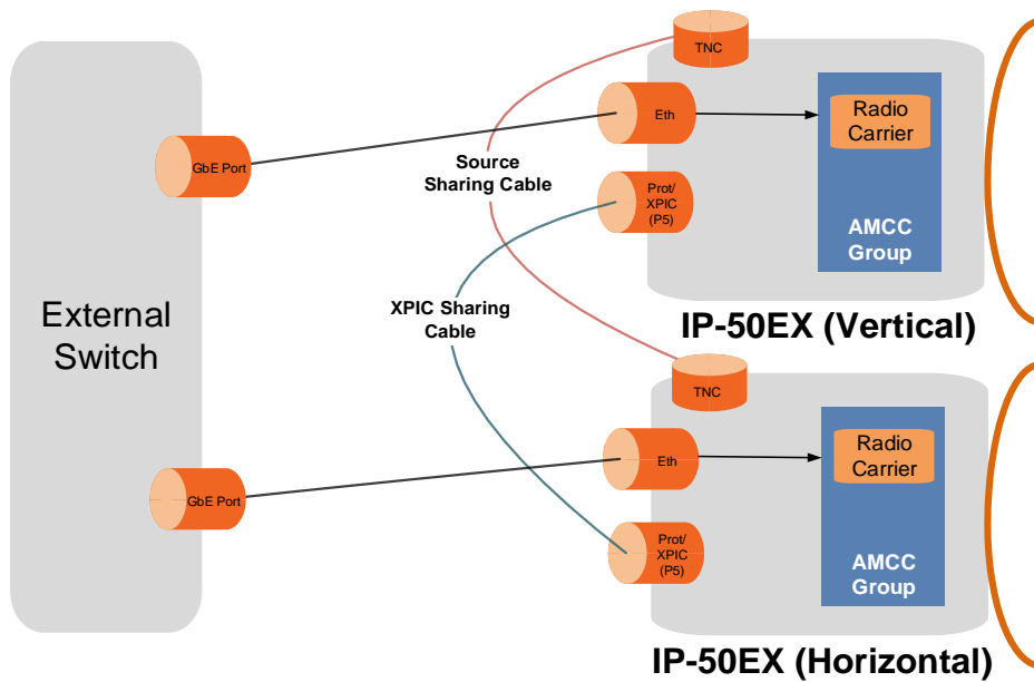
Figure 25: 2+0 XPIC Configuration – Integrated Antenna
