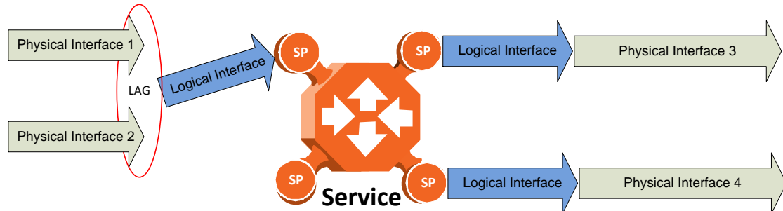
Figure 40: Grouped Interfaces as a Single Logical Interface on Ingress Side
