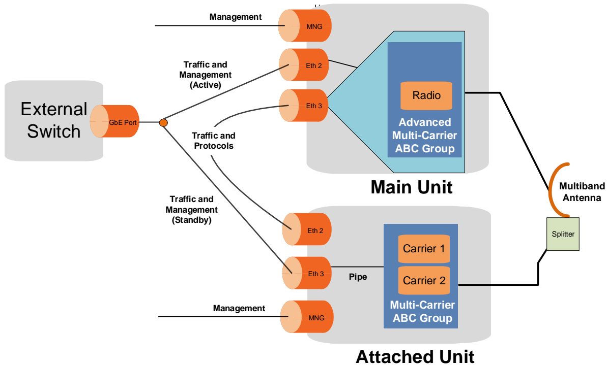
Figure 19: Layer 1 Link Aggregation with Line Redundancy (Multiband with Multiband Antenna)
