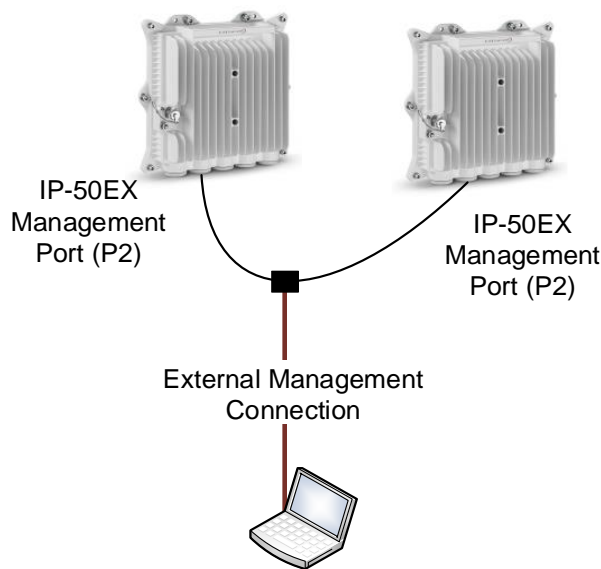
Figure 27: Unit Redundancy Local Management
