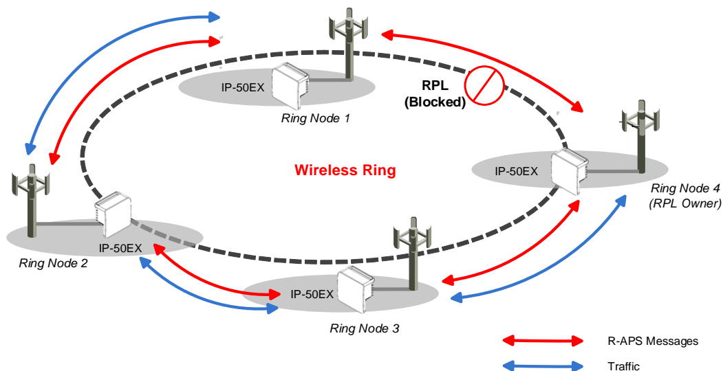
Figure 49: G.8032 Ring in Idle (Normal) State
