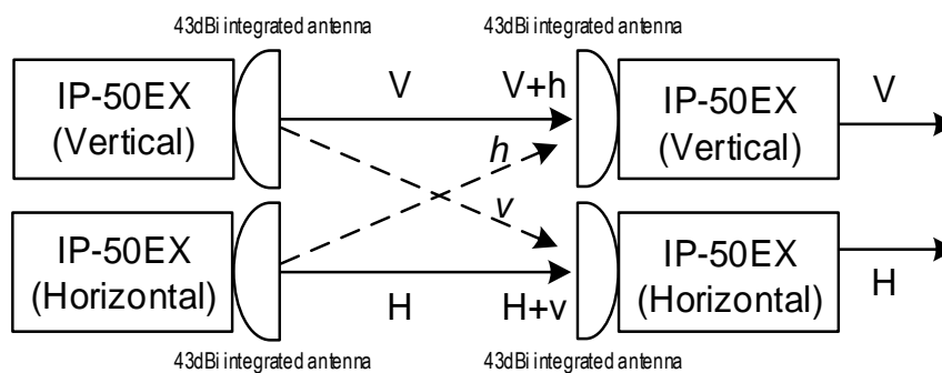
Figure 22: XPIC Implementation – Integrated Antenna
