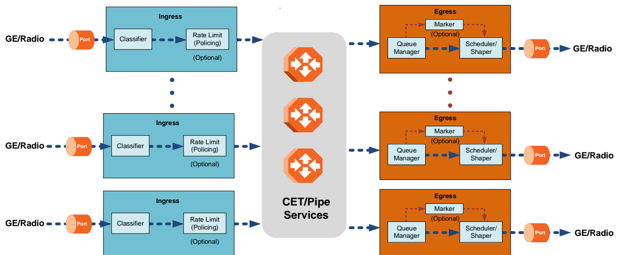
Figure 43: QoS Block Diagram
