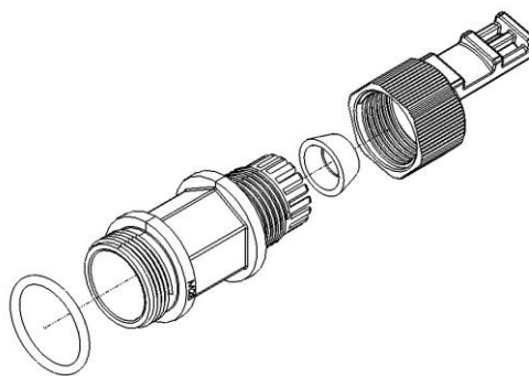
Figure 7: Cable Gland Construction
