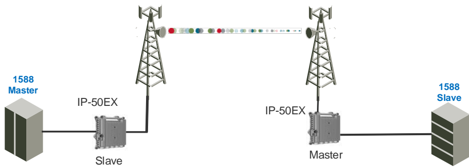
Figure 58: Boundary Clock – General Architecture
