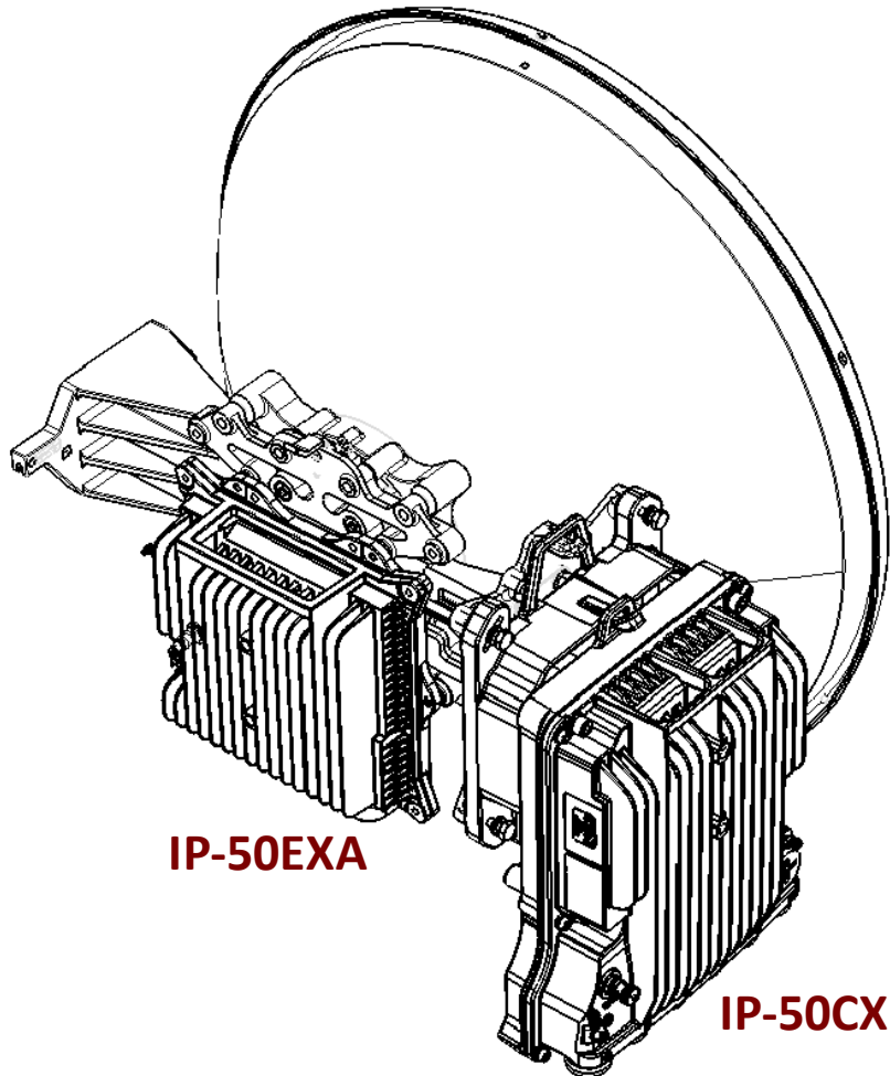
Figure 5: Multiband with IP-50EXA and IP-50CX
