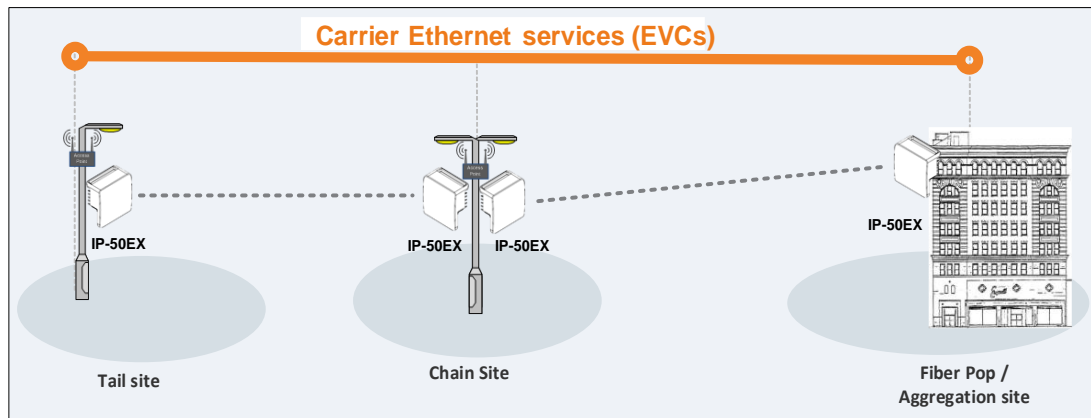
Figure 52: IP-50EX End-to-End Service Management
