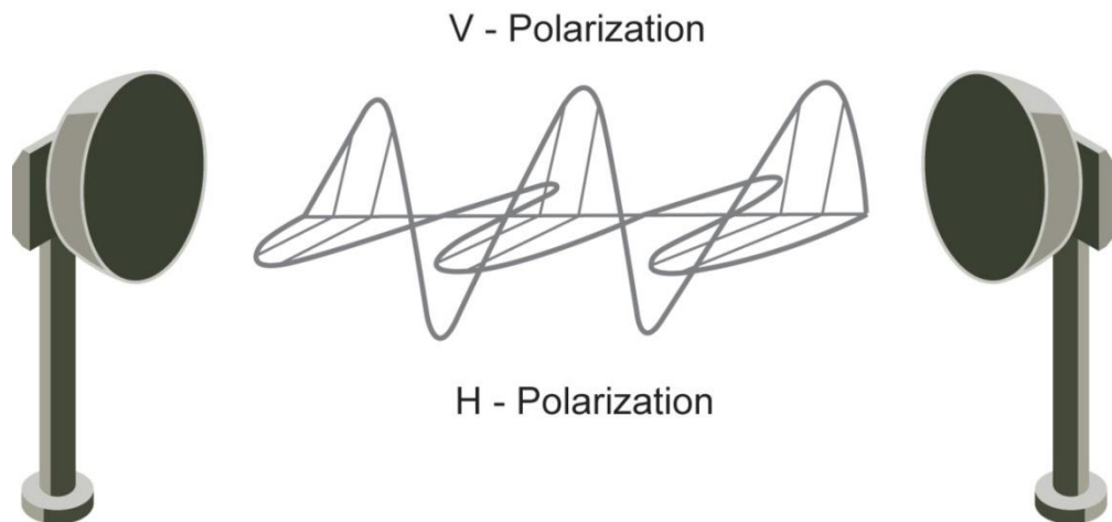
Figure 20: Dual Polarization
