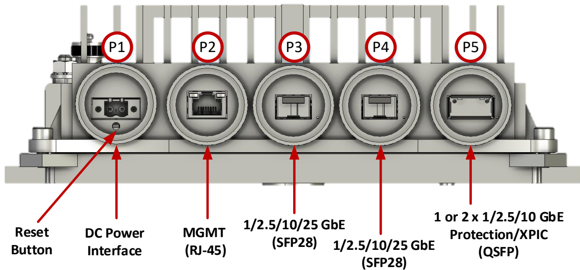
Figure 10: IP-50EXA Interfaces
