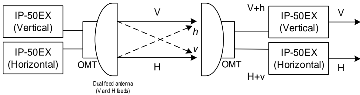
Figure 21: XPIC Implementation – Direct Mount
