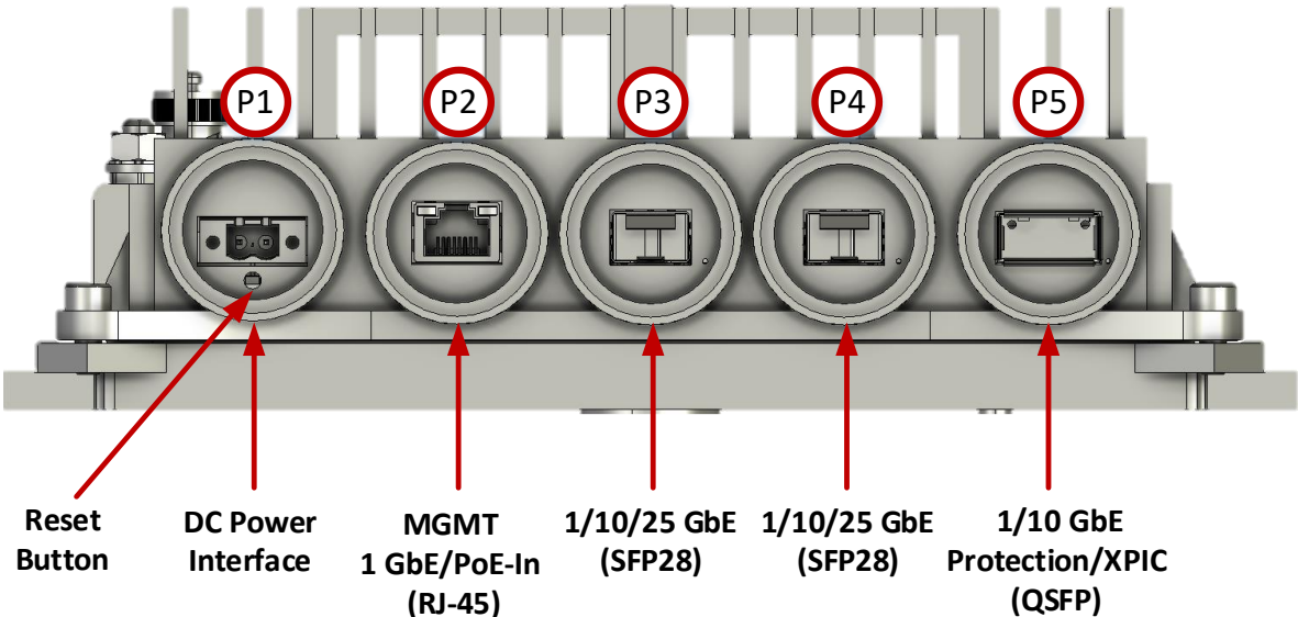
Figure 9: IP-50EX-P Interfaces
