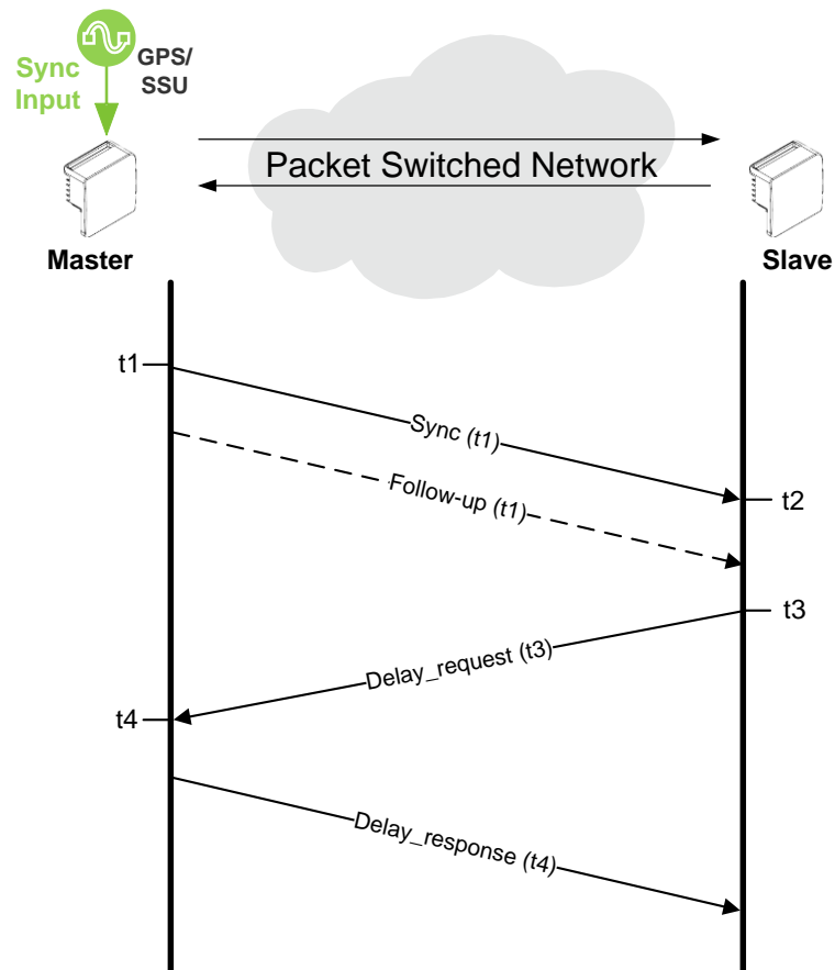
Figure 55: Calculating the Propagation Delay for PTP Packets
