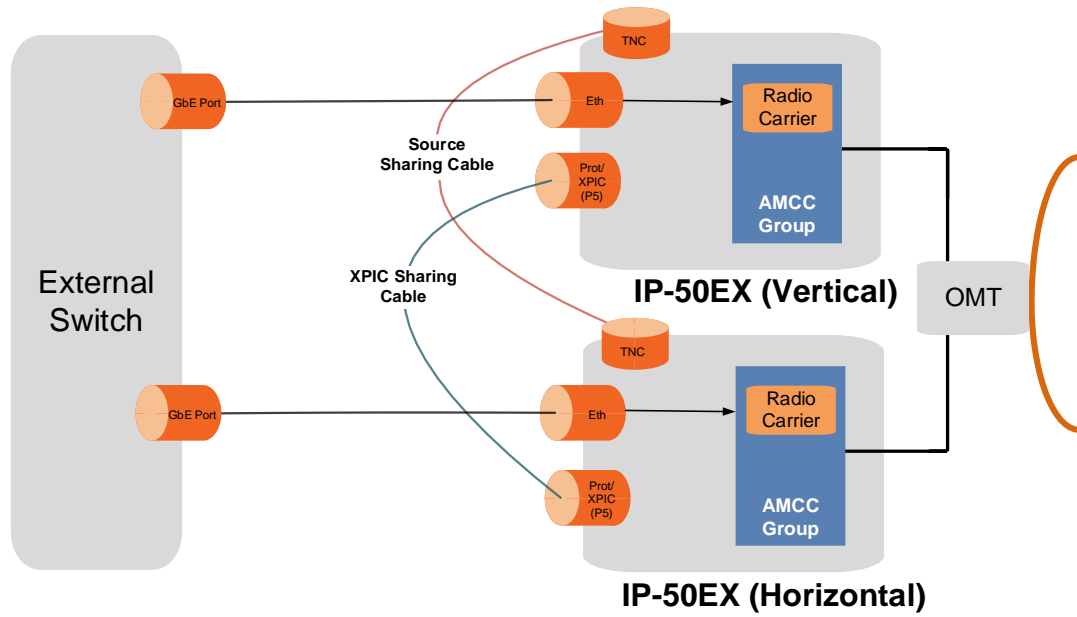
Figure 24: 2+0 XPIC Configuration – Direct Mount
