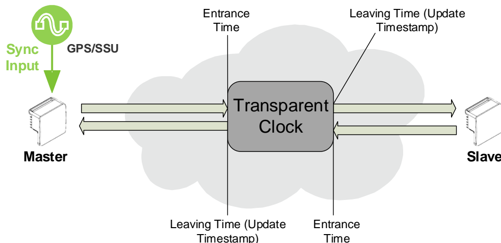
Figure 56: Transparent Clock – General Architecture
