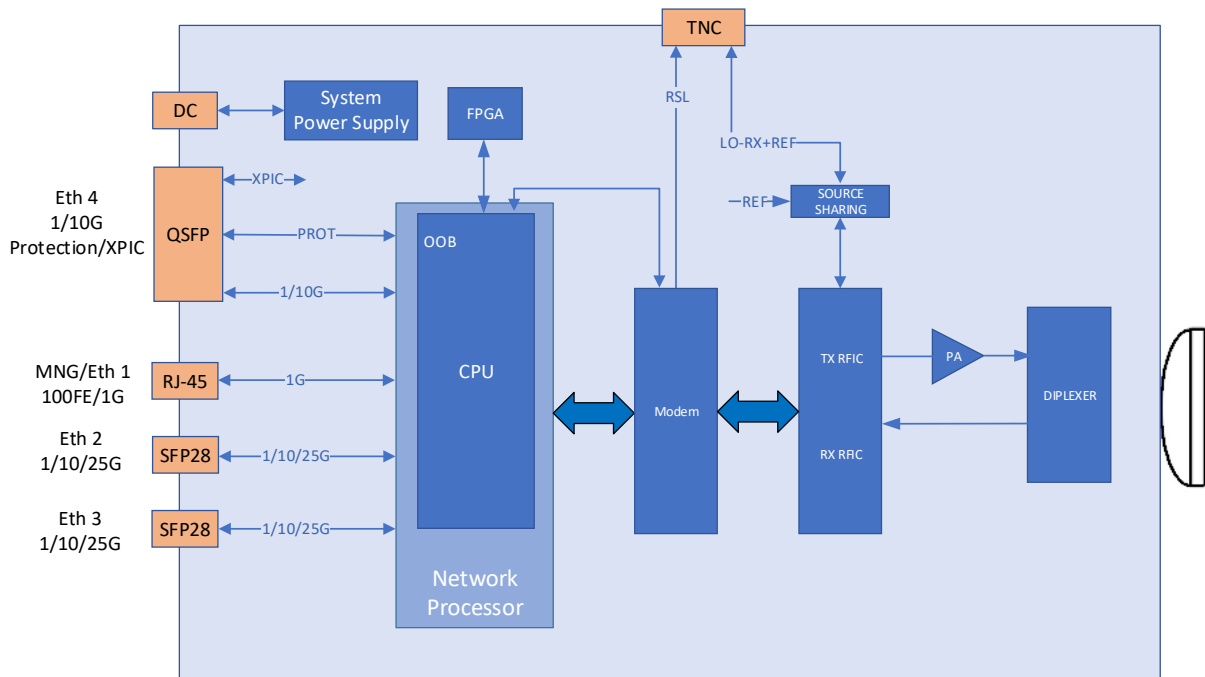
Figure 12: IP-50EX-P Block Diagram
