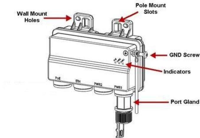
Figure 7: PoE Injector
