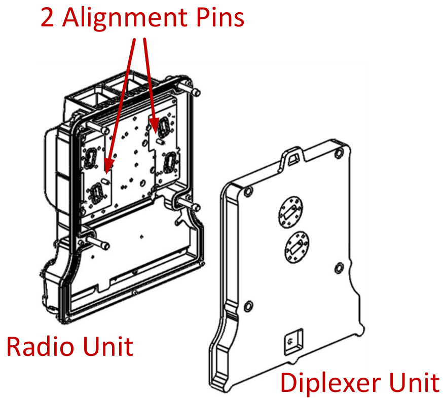
Figure 25: Attaching the Diplexer
