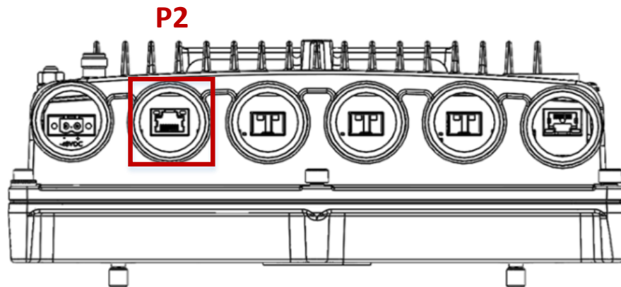
Figure 28: Protocols Cable – IP-50C (with IP-20C ESS or IP-20C-HP)
