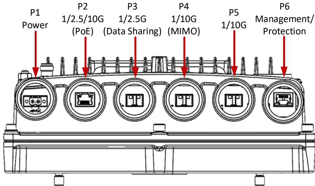
Figure 3: IP-50C Interfaces
