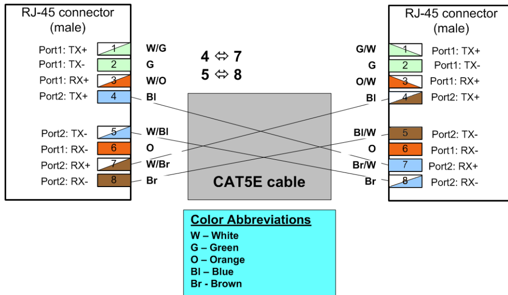
Figure 21: MIMO/Protection Signaling Cable Pinouts
