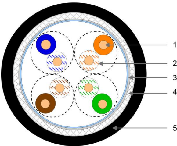
Figure 18: Cable Design
