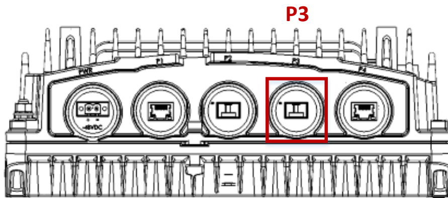
Figure 31: Protocols Cable – IP-20C (ESX)
