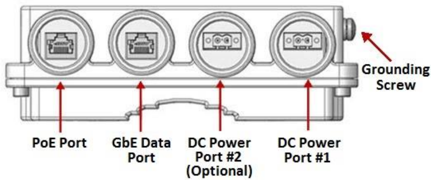
Figure 8: PoE Injector Ports
