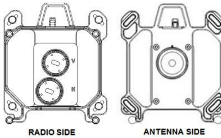
Figure 6: OMT
