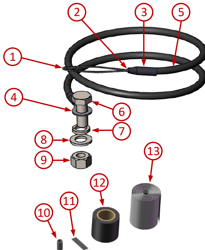
Figure 17: Cable Grounding Kit
