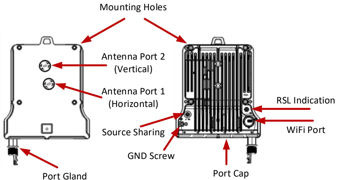
Figure 1: IP-50C Rear View (Left) and Front View (Right)
