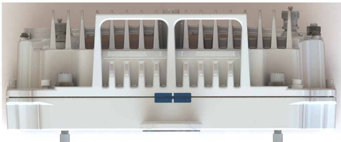
Figure 36: Applying Tamper-Evident FIPS Labels – IP-50C – Left Side
