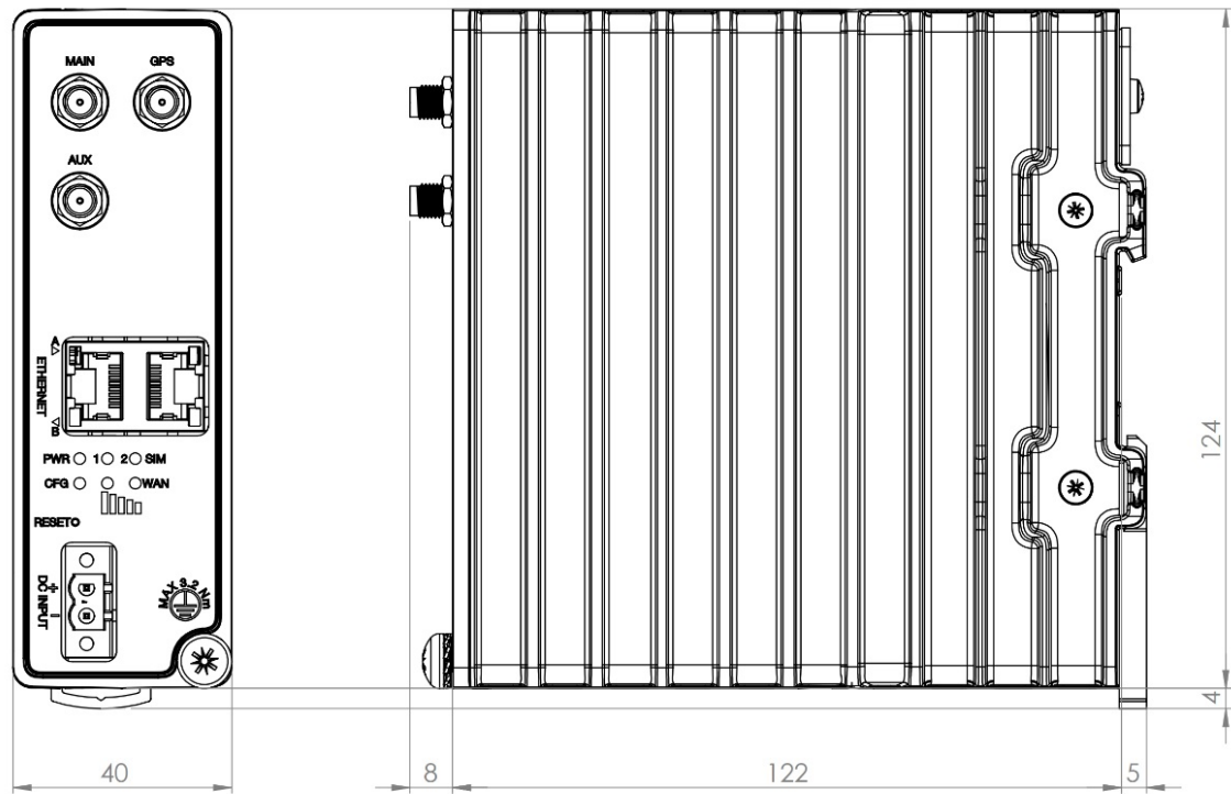
Figure 5. Dimensional drawing
