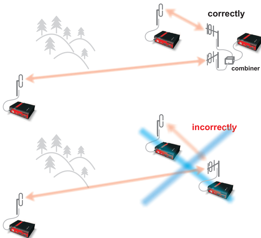
Fig. 3.5: Main lobe
