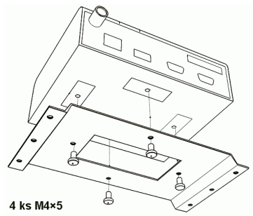
Fig. 6.7: Vertical lengthwise mounting to DIN rail
