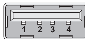
Fig. 4.12: Serial connector
