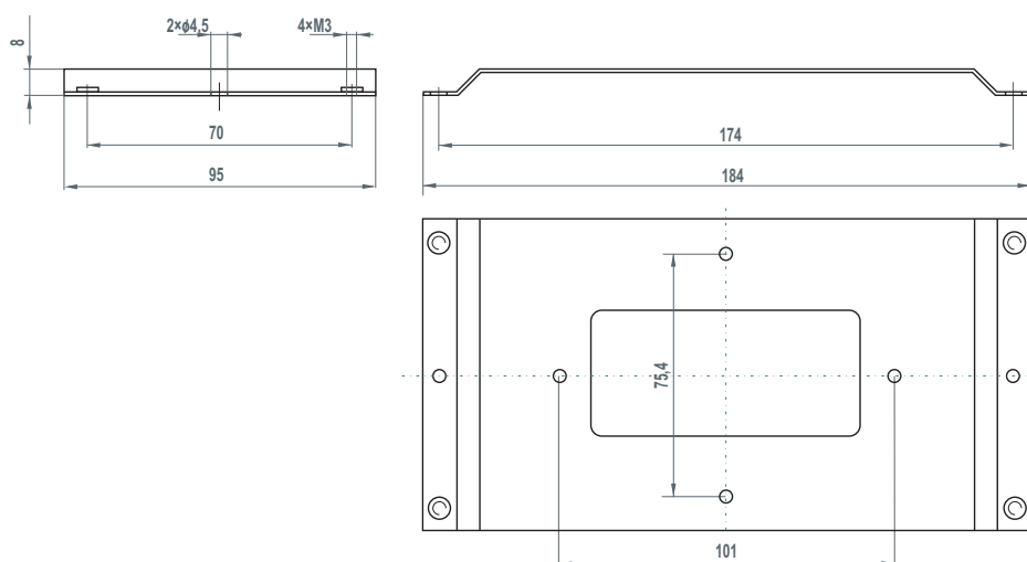
Fig. 4.25: Flat-bracket dimensions
