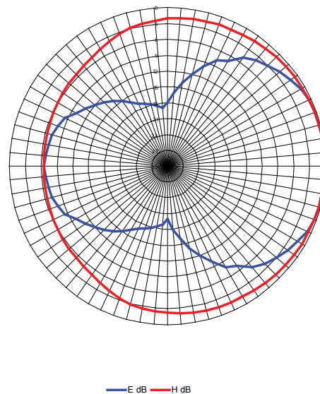
RADIATION PATTERN
